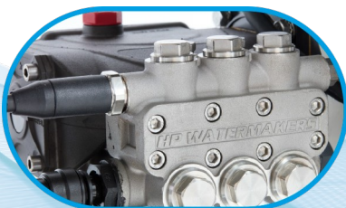
High Pressure Pump (6000 hours before maintenance)
